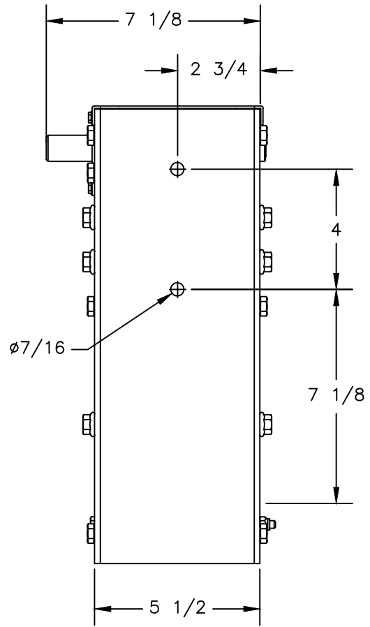
SIDE VIEW (MOUNTING HOLE PATTERN SAME ON BOTH SIDES)
