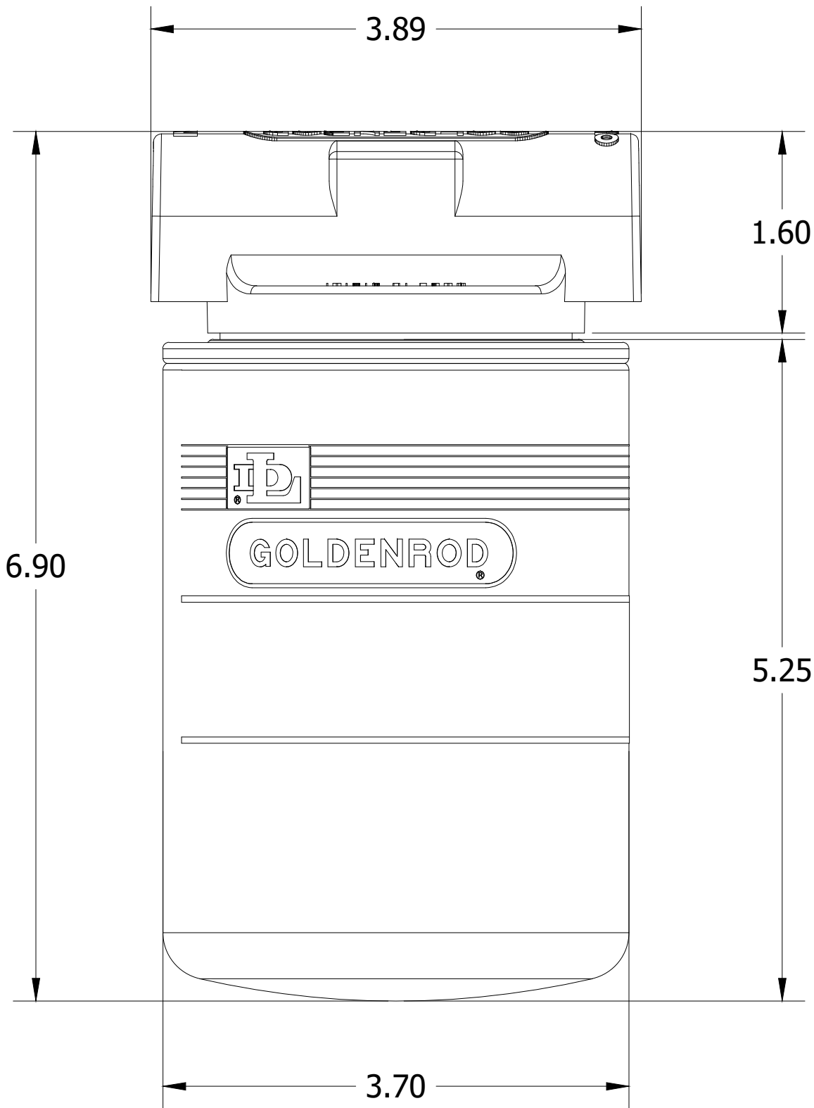
596-3/4 FUEL FILTER ASSY
