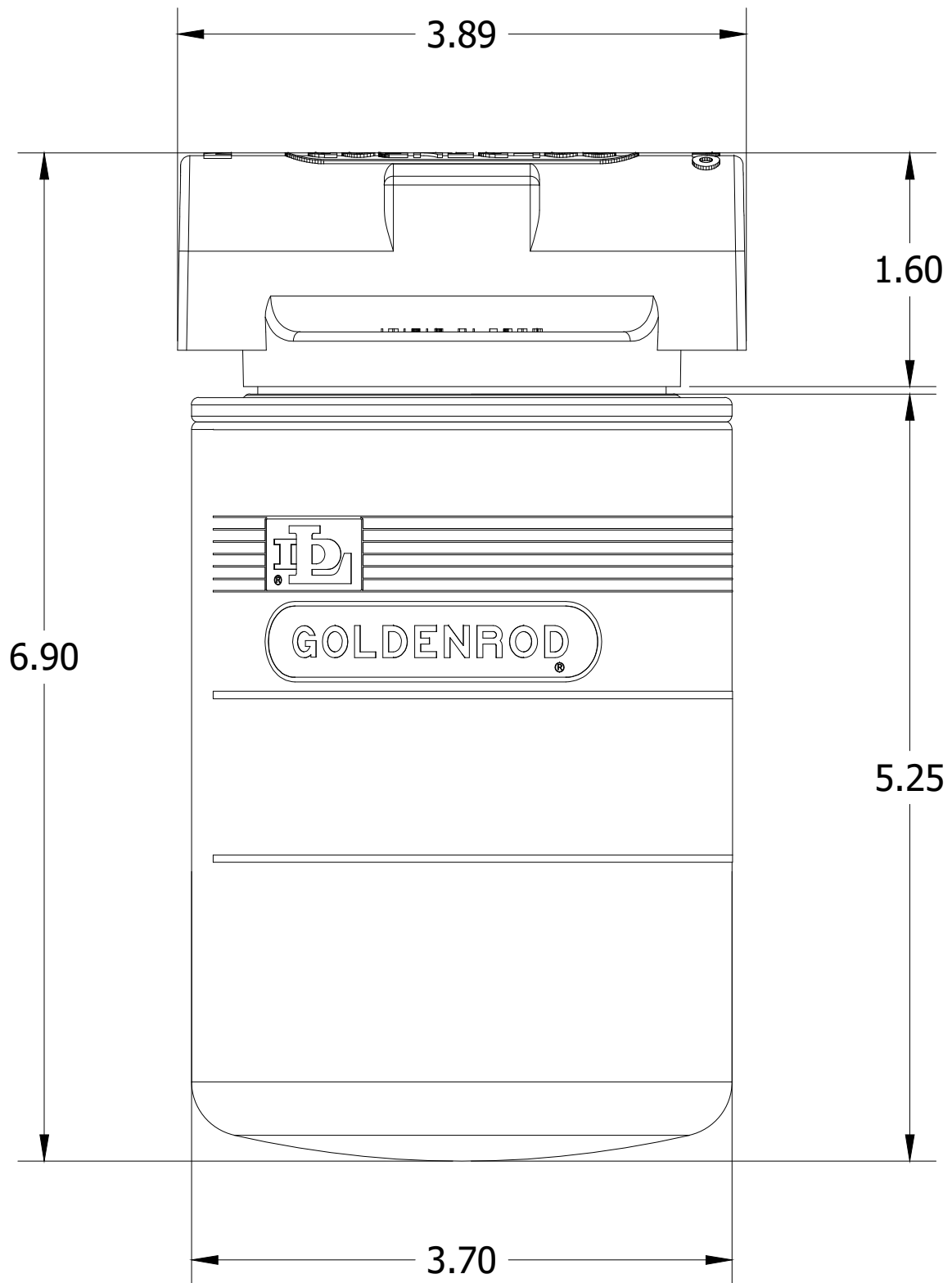
595-3/4 FUEL FILTER ASSY
